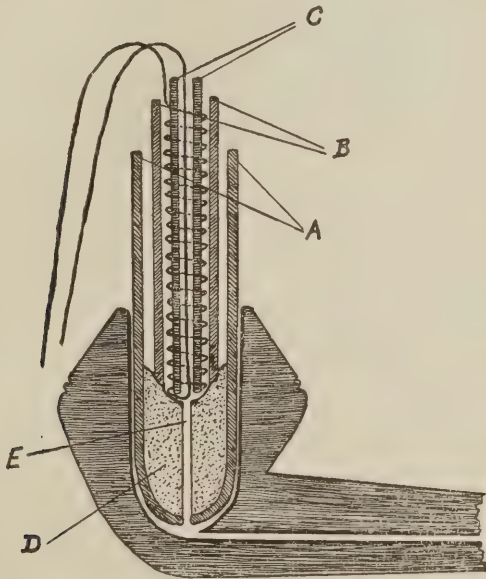
PLATE 3. Diagram of experimental pipe. A , aluminum capsule; B , outer asbestos tube; C , inner asbestos tube; D , plaster moistened with water; E , hole through moistened plaster through which heated air passes.
